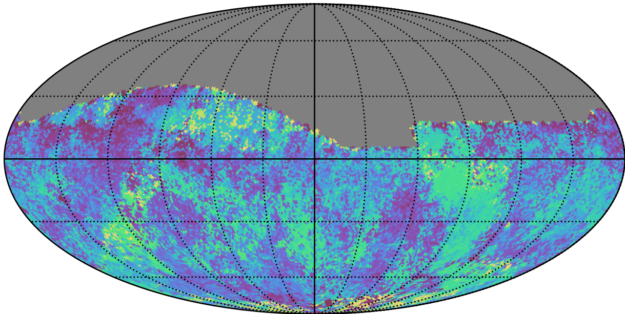
too_10_1v3.4_10yrs Yr 1 all bands: Median skyBrightness
