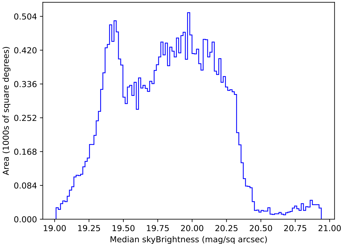
too_10_1v3.4_10yrs Yr 1 all bands: Median skyBrightness
