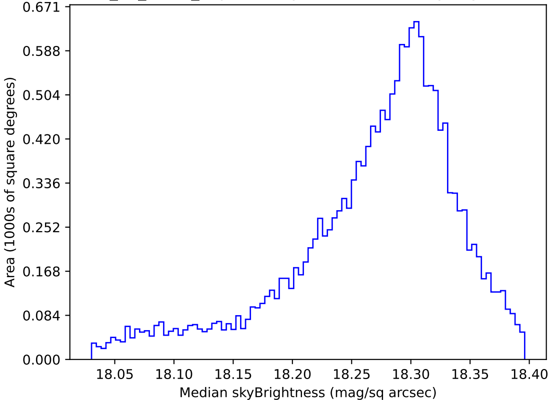
too_10_1v3.4_10yrs WFD y band: Median skyBrightness
