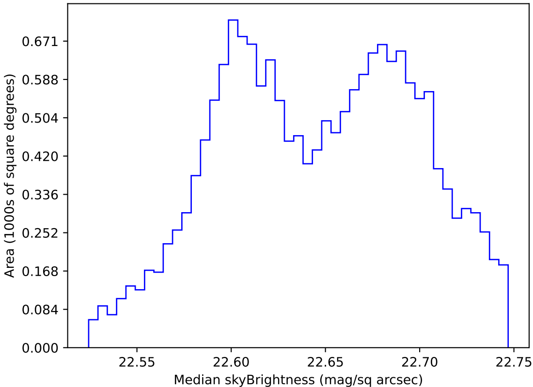
too_10_1v3.4_10yrs WFD u band: Median skyBrightness
