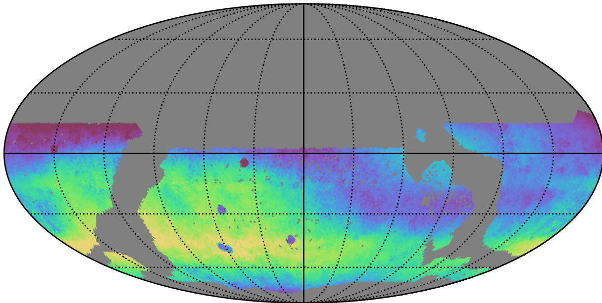
too_10_1v3.4_10yrs WFD r band: Median skyBrightness
