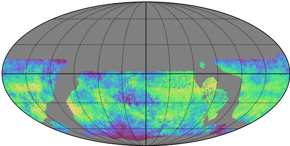
too_10_1v3.4_10yrs WFD i band: Median skyBrightness
