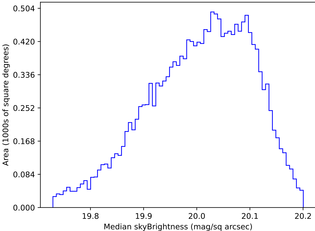
too_10_1v3.4_10yrs WFD i band: Median skyBrightness
