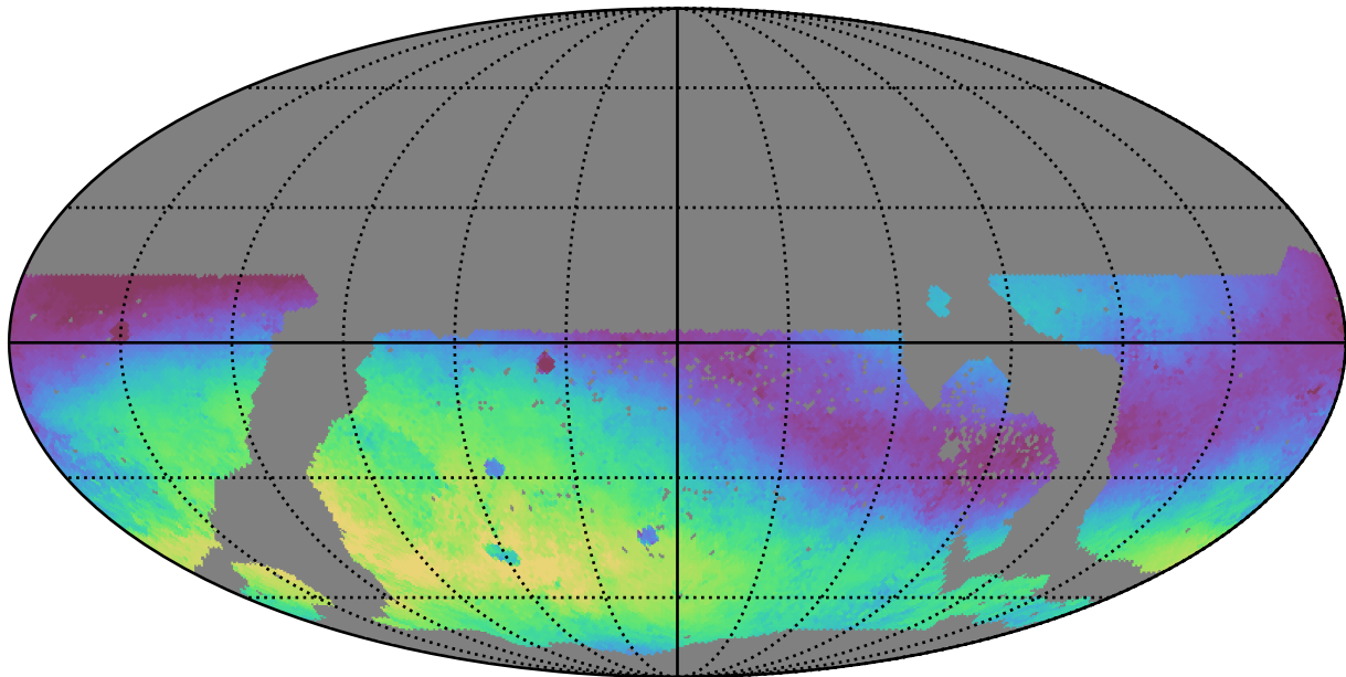
too_10_1v3.4_10yrs WFD g band: Median skyBrightness
