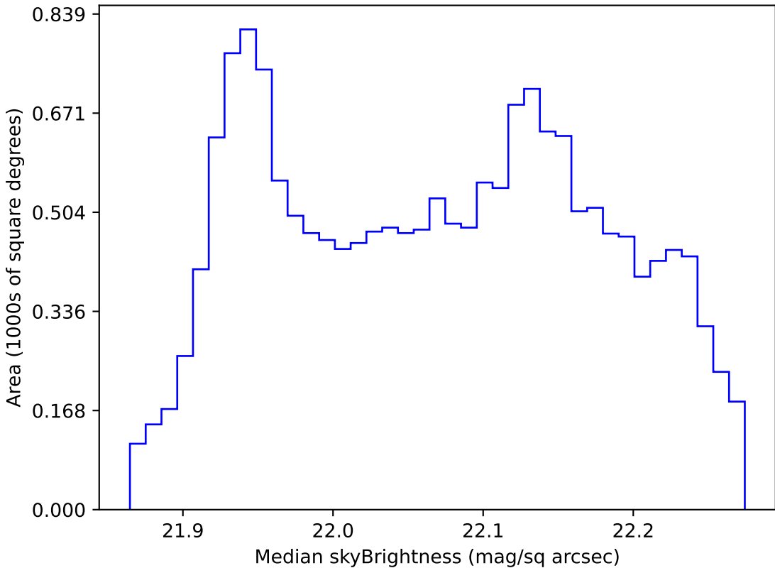
too_10_1v3.4_10yrs WFD g band: Median skyBrightness
