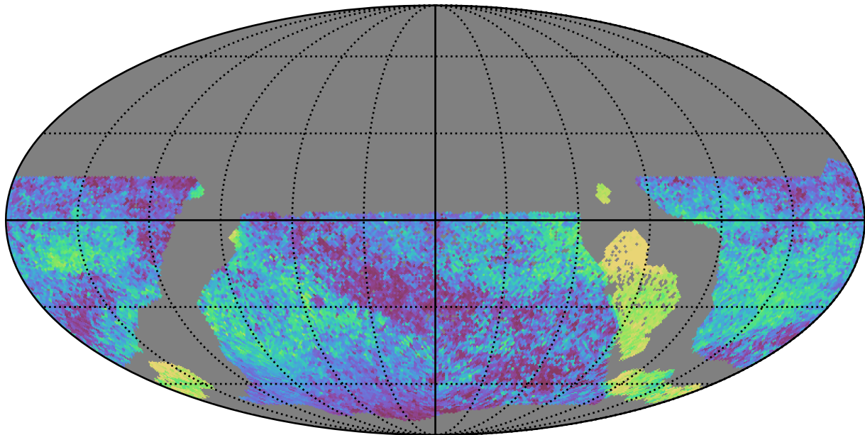
too_10_1v3.4_10yrs WFD all bands: Median skyBrightness
