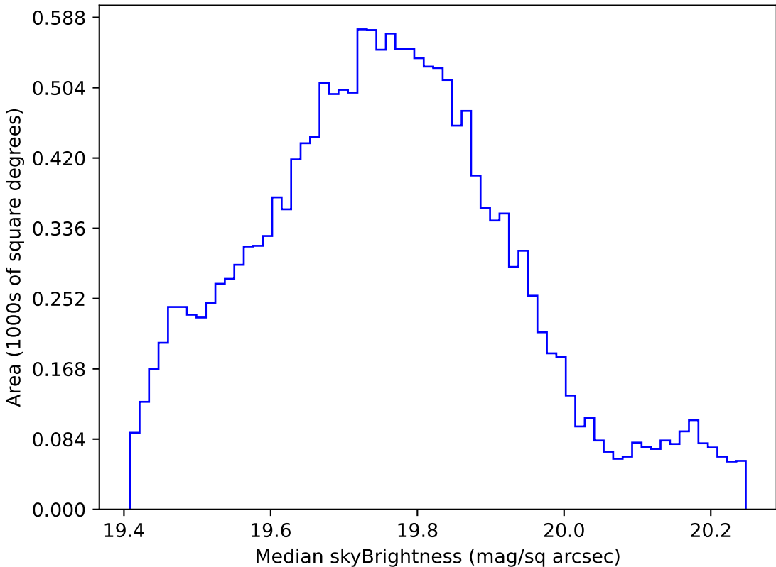
too_10_1v3.4_10yrs WFD all bands: Median skyBrightness
