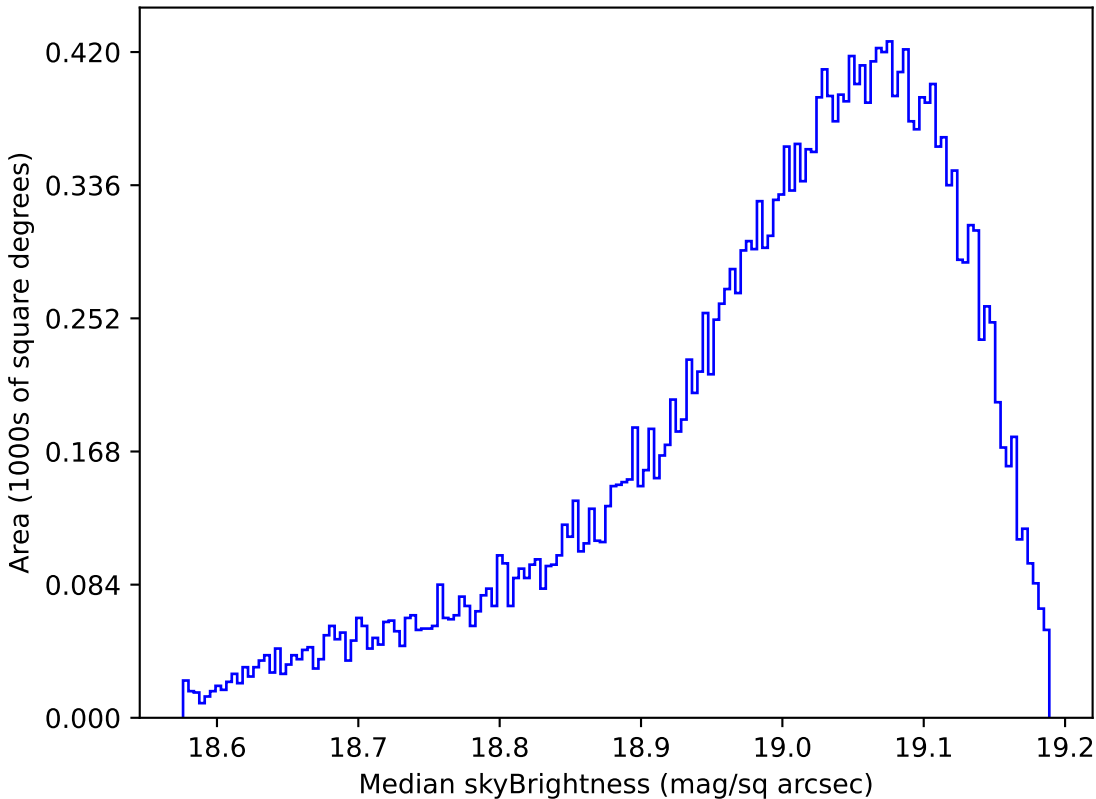
too_10_1v3.4_10yrs All sky z band: Median skyBrightness
