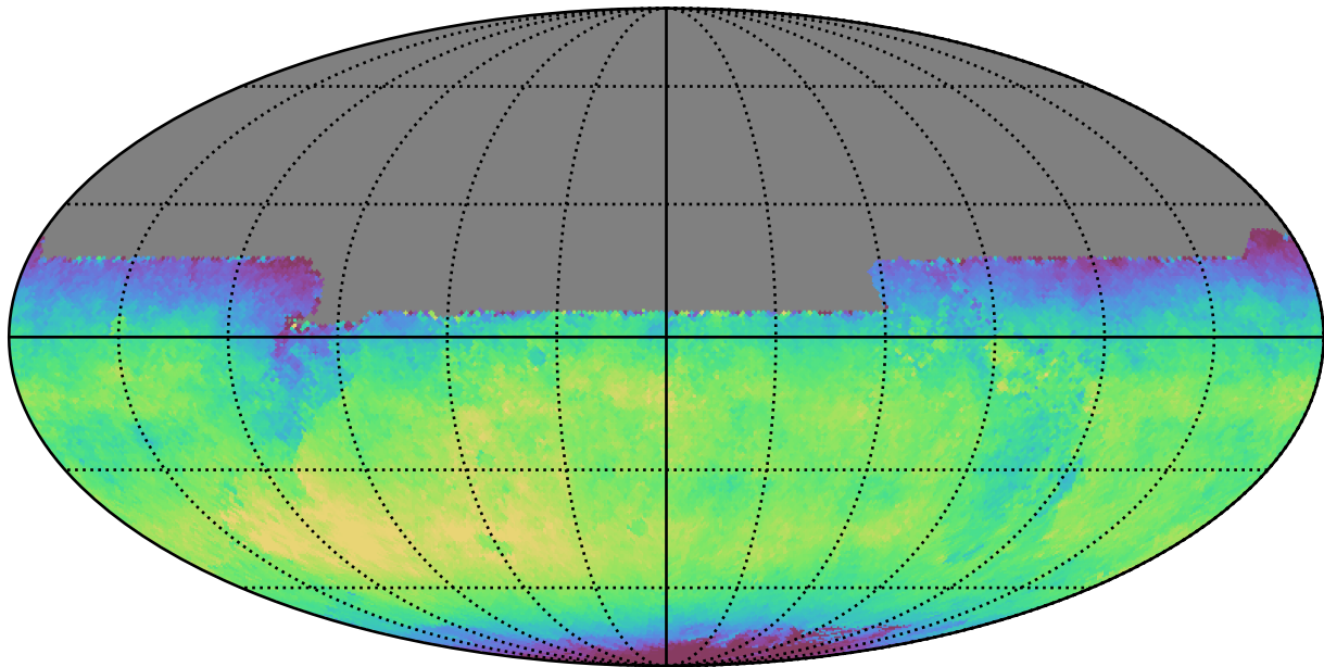
too_10_1v3.4_10yrs All sky y band: Median skyBrightness
