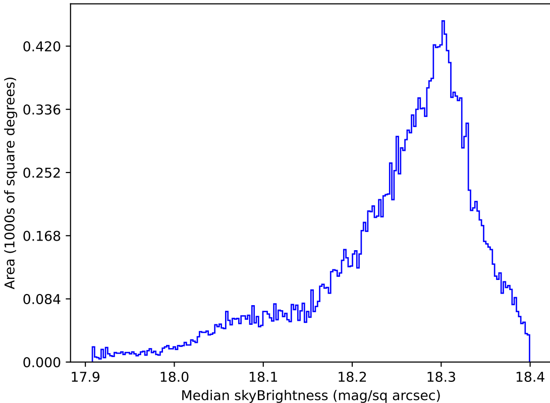
too_10_1v3.4_10yrs All sky y band: Median skyBrightness
