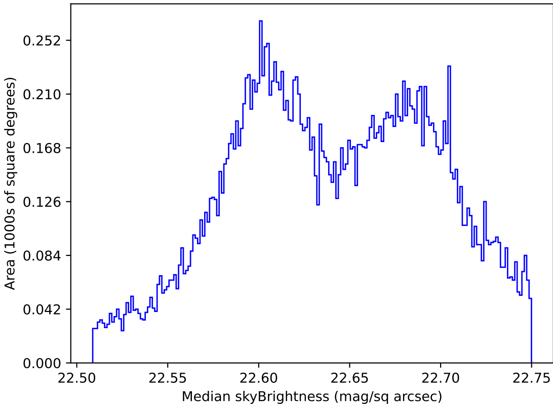
too_10_1v3.4_10yrs All sky u band: Median skyBrightness
