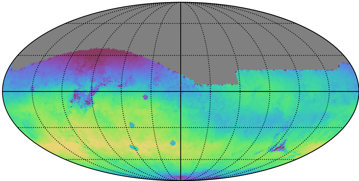
too_10_1v3.4_10yrs All sky r band: Median skyBrightness
