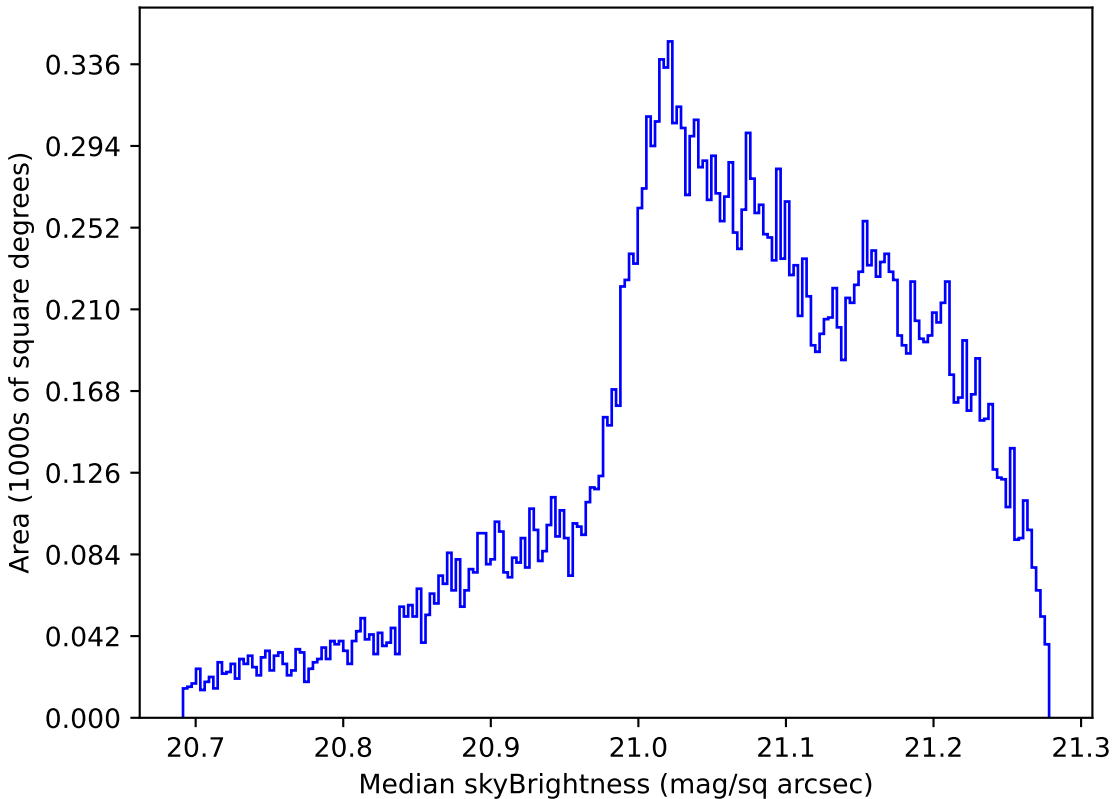
too_10_1v3.4_10yrs All sky r band: Median skyBrightness
