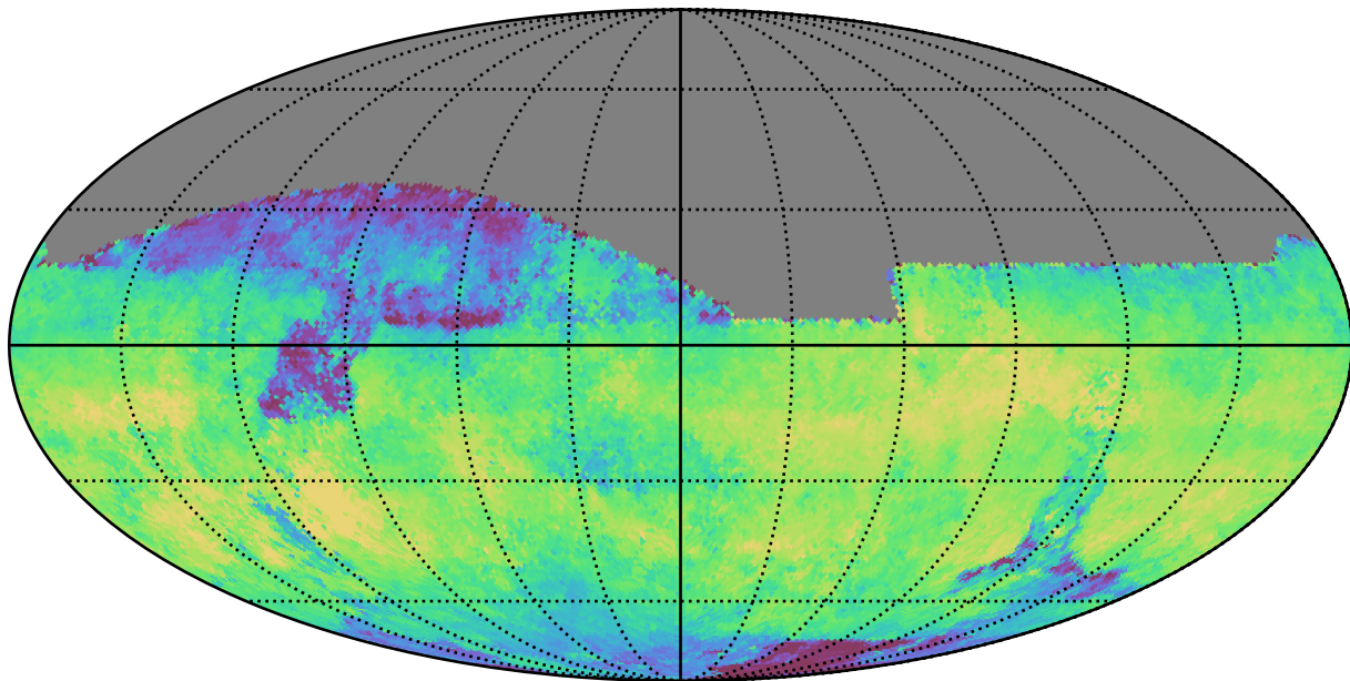
too_10_1v3.4_10yrs All sky i band: Median skyBrightness
