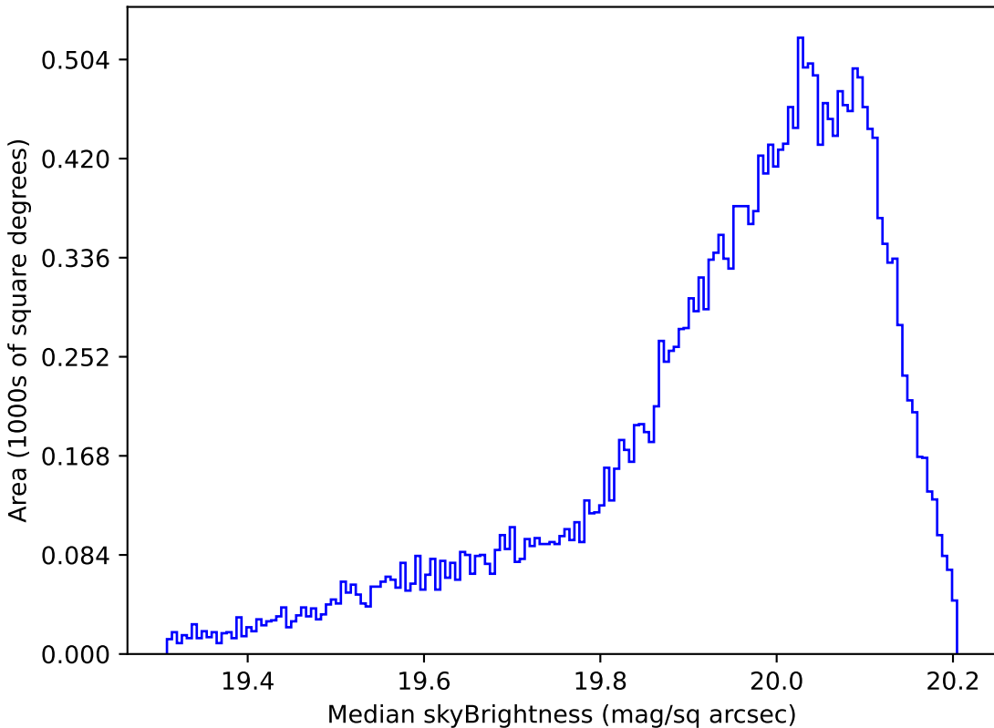
too_10_1v3.4_10yrs All sky i band: Median skyBrightness
