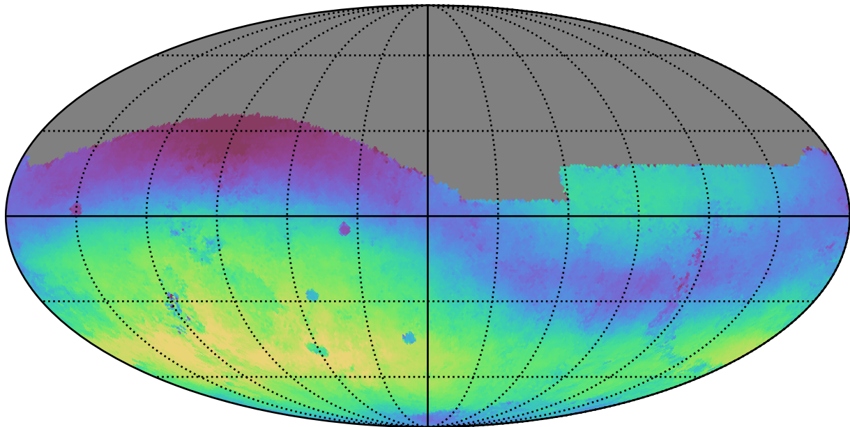
too_10_1v3.4_10yrs All sky g band: Median skyBrightness
