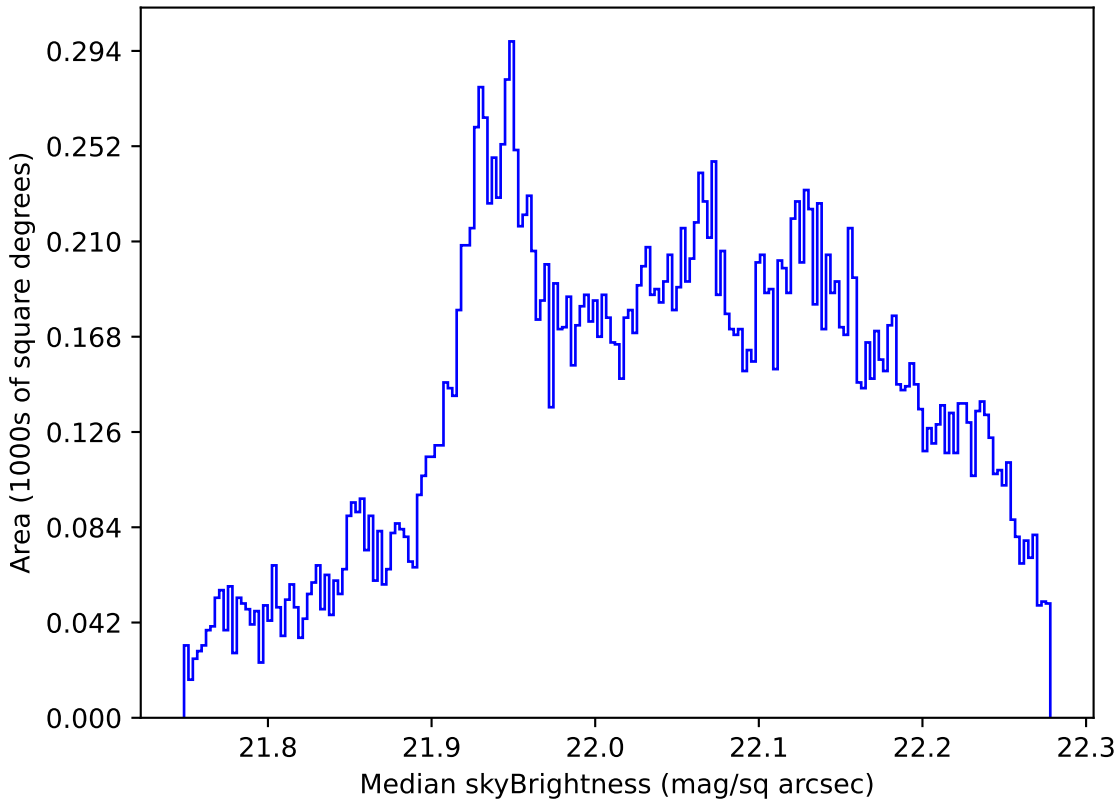
too_10_1v3.4_10yrs All sky g band: Median skyBrightness
