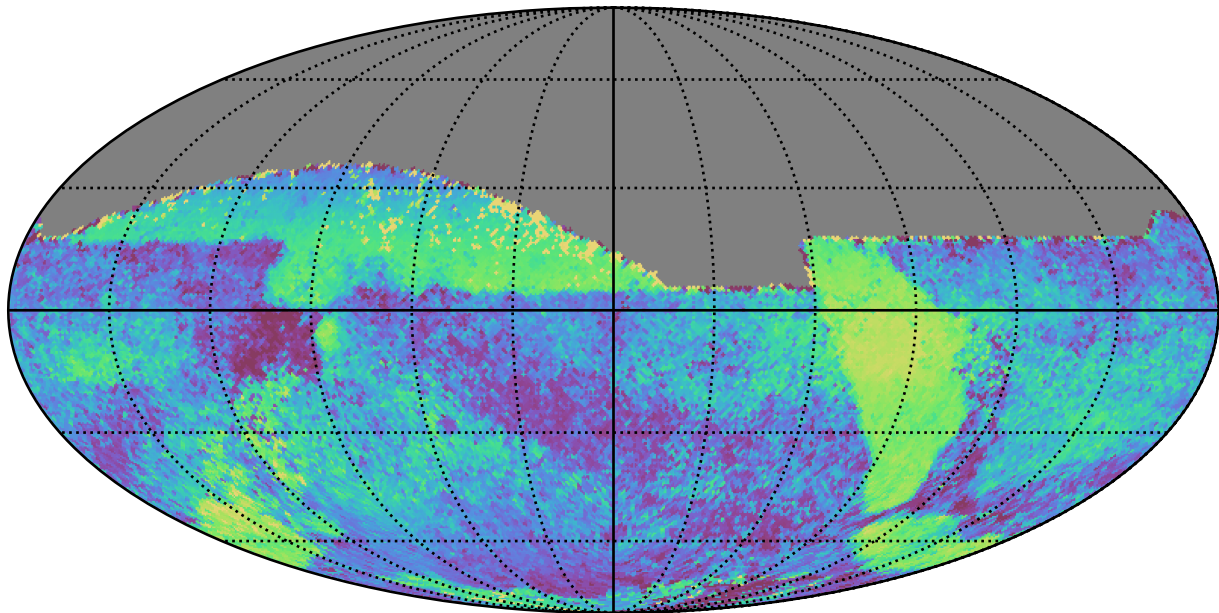
too_10_1v3.4_10yrs All sky all bands: Median skyBrightness
