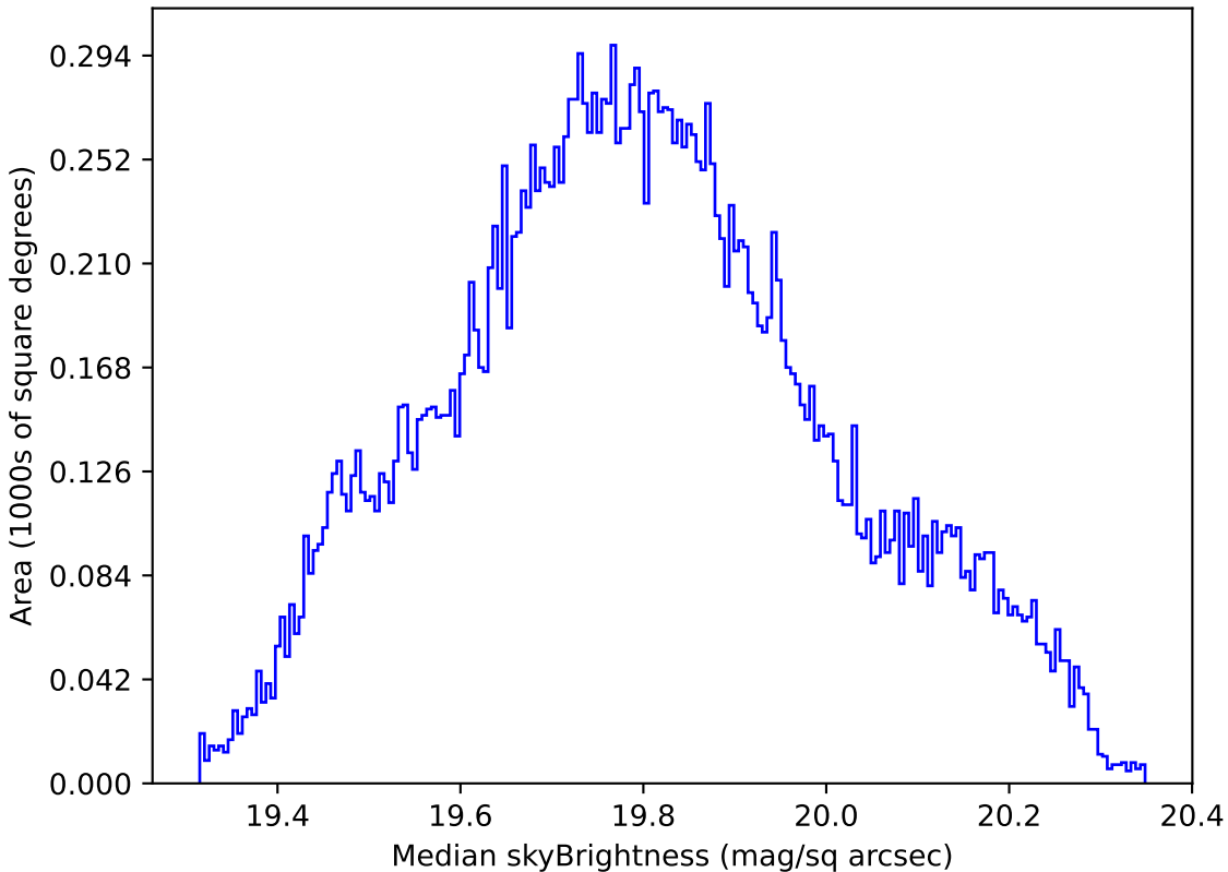
too_10_1v3.4_10yrs All sky all bands: Median skyBrightness
