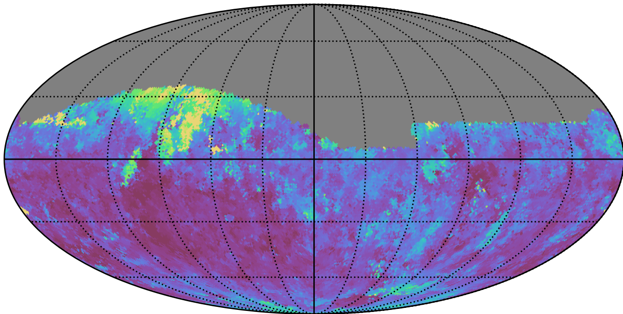
too_10_1v3.4_10yrs Yr 1 z band: Median seeingGeom
