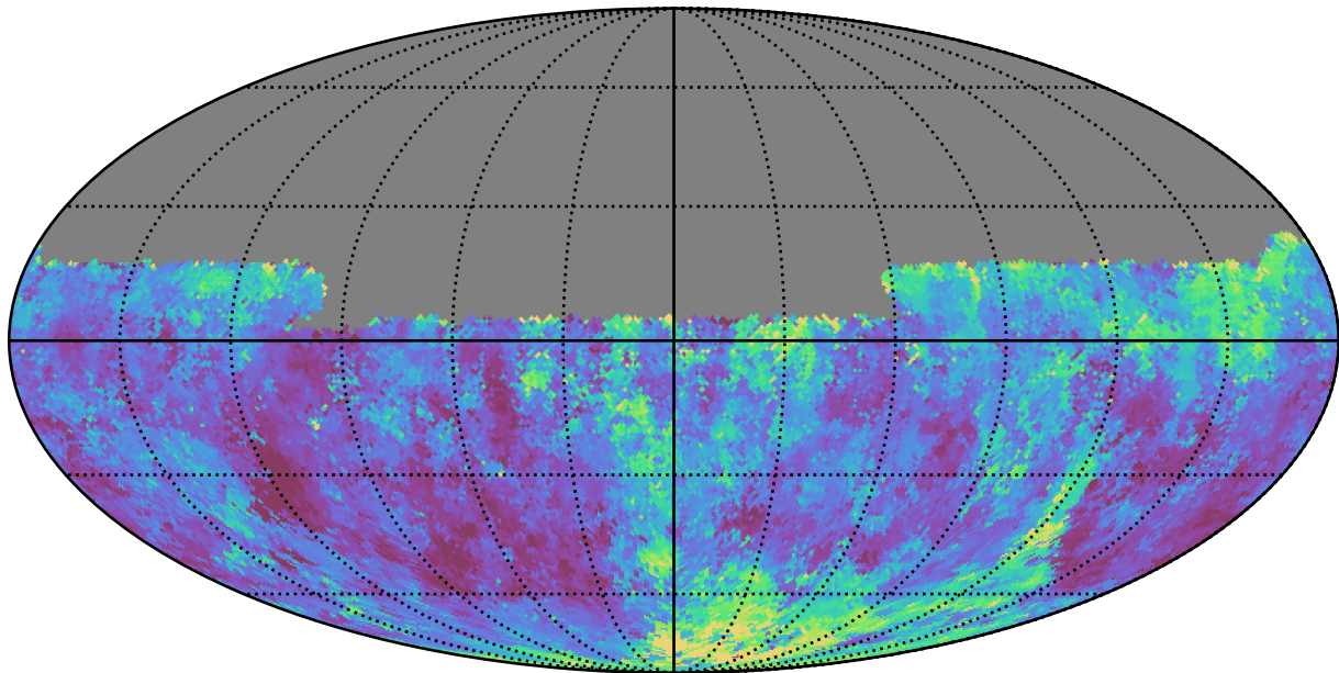
too_10_1v3.4_10yrs Yr 1 y band: Median seeingGeom
