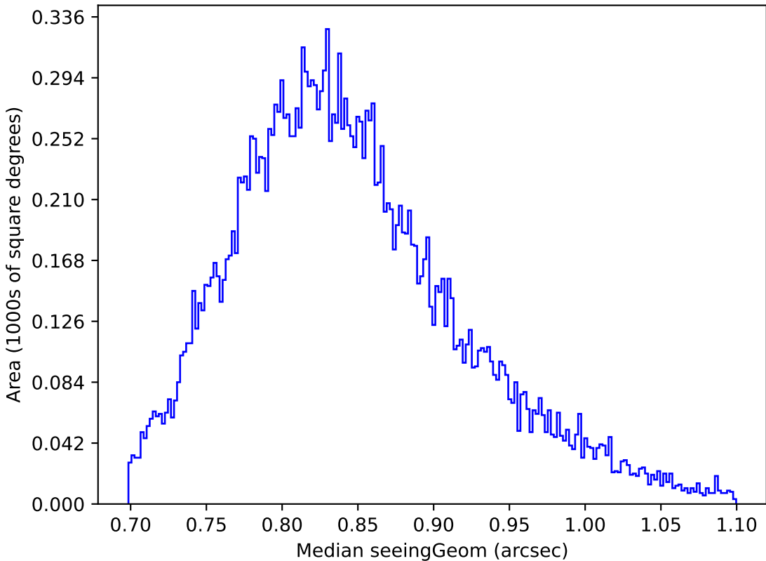
too_10_1v3.4_10yrs Yr 1 y band: Median seeingGeom
