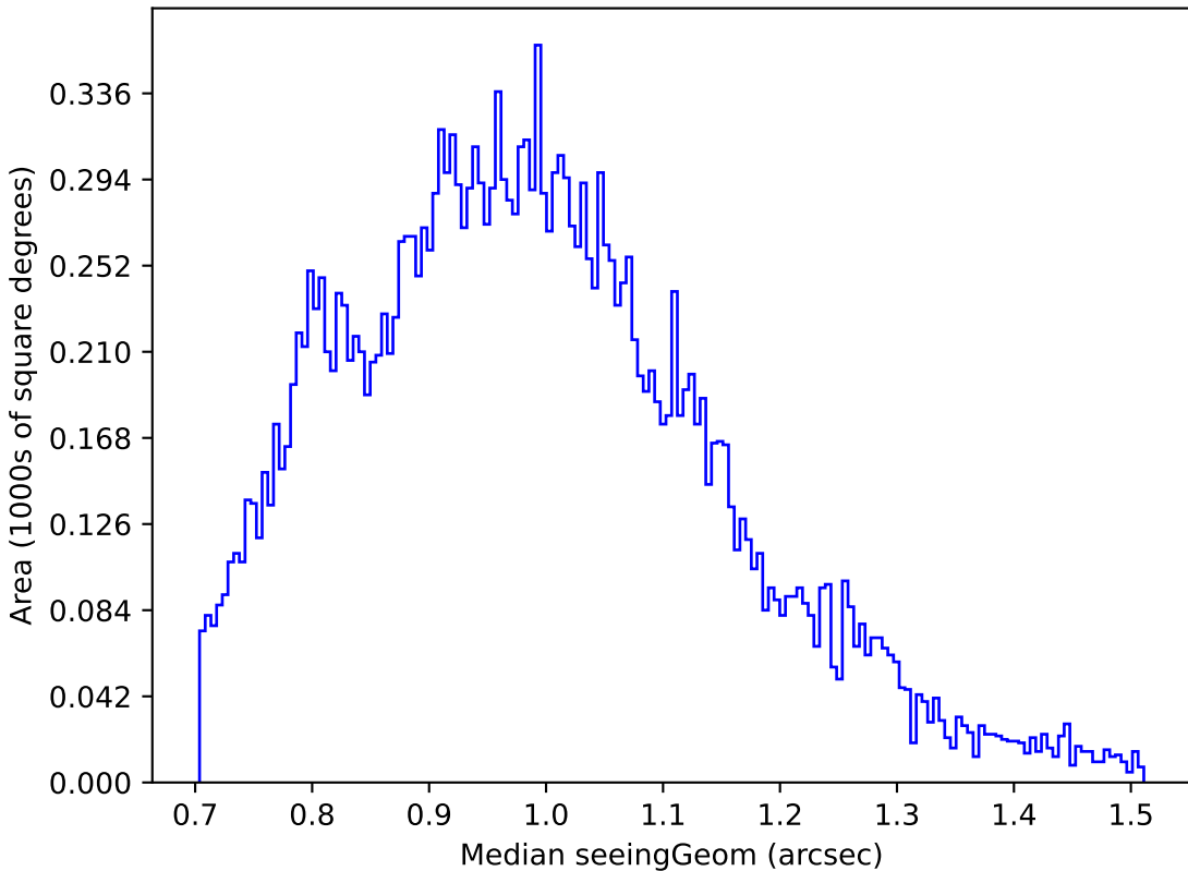
too_10_1v3.4_10yrs Yr 1 u band: Median seeingGeom
