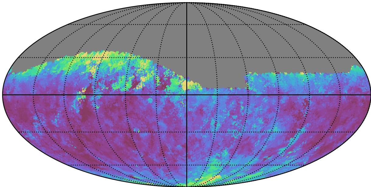
too_10_1v3.4_10yrs Yr 1 r band: Median seeingGeom
