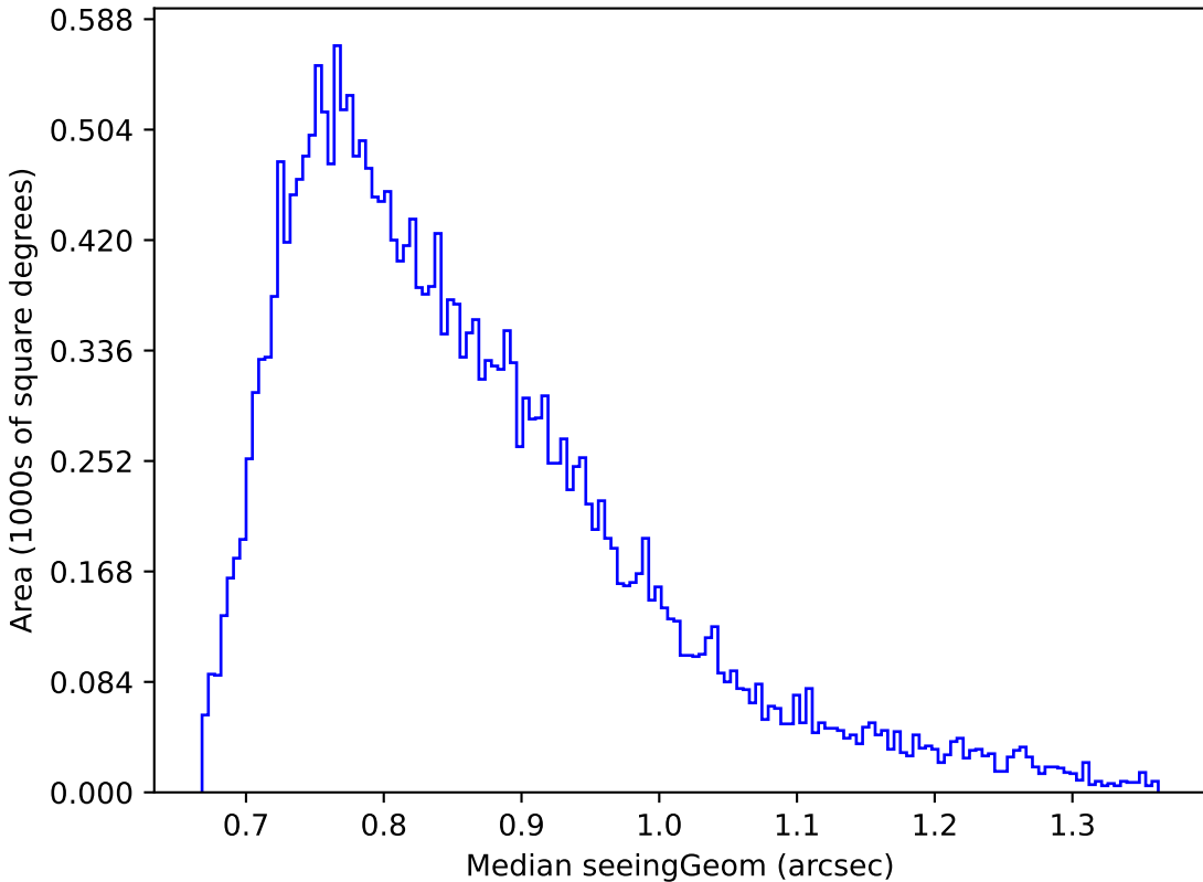
too_10_1v3.4_10yrs Yr 1 r band: Median seeingGeom
