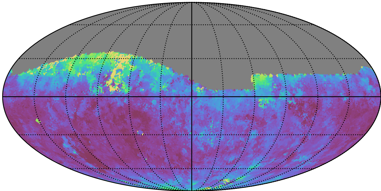
too_10_1v3.4_10yrs Yr 1 i band: Median seeingGeom
