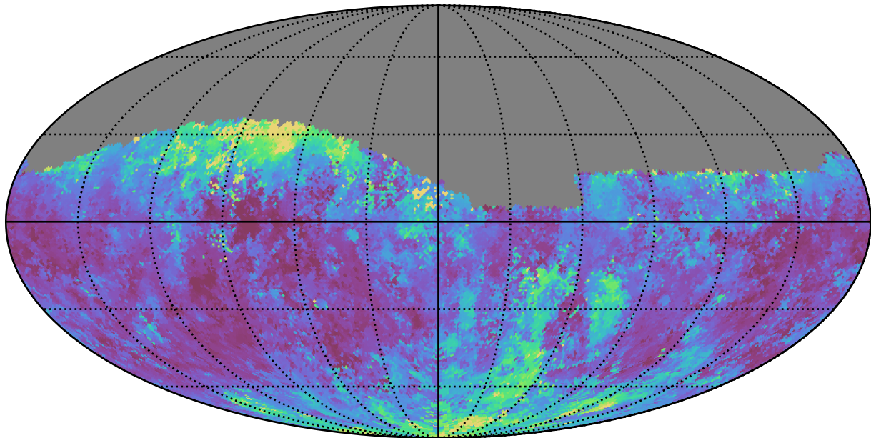
too_10_1v3.4_10yrs Yr 1 g band: Median seeingGeom
