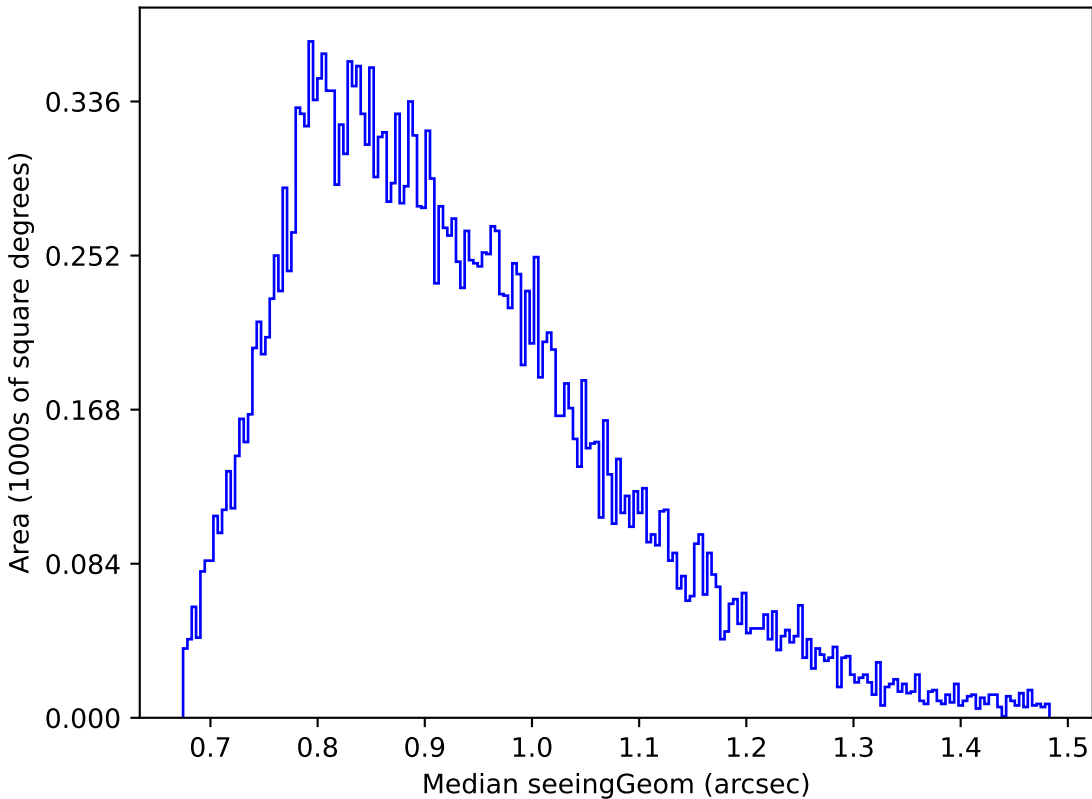
too_10_1v3.4_10yrs Yr 1 g band: Median seeingGeom
