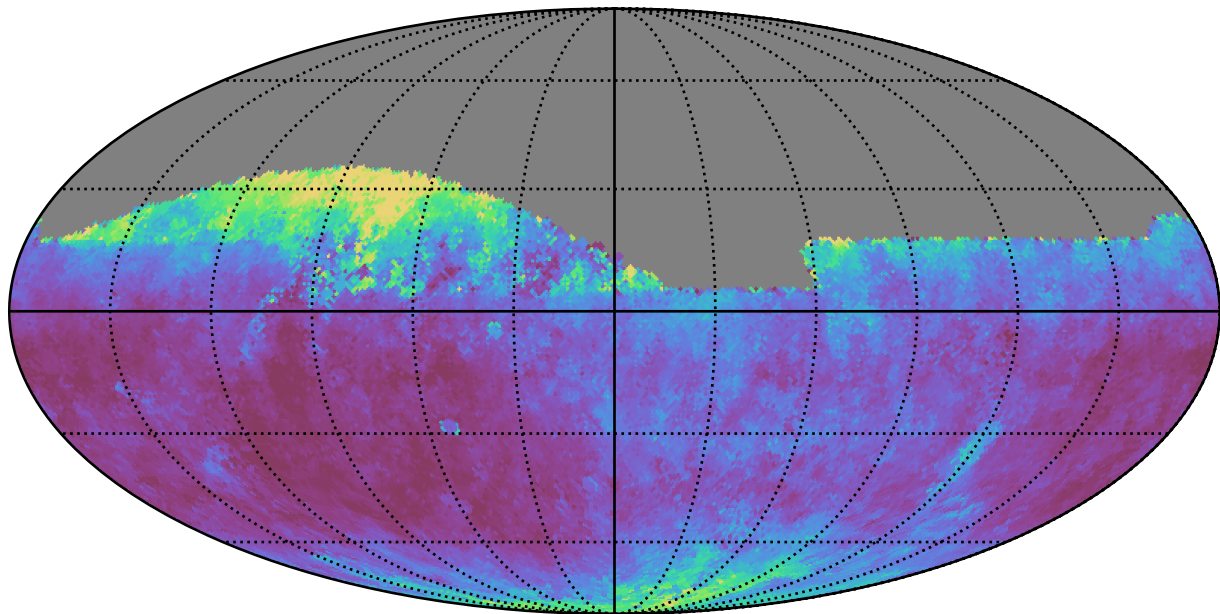
too_10_1v3.4_10yrs Yr 1 all bands: Median seeingGeom
