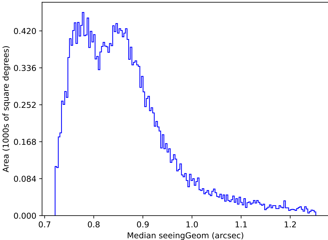
too_10_1v3.4_10yrs Yr 1 all bands: Median seeingGeom
