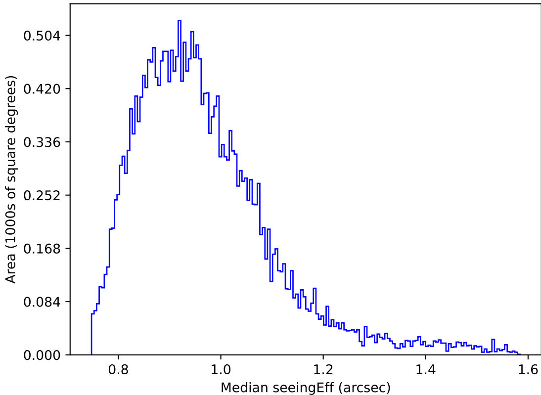
too_10_1v3.4_10yrs Yr 1 z band: Median seeingEff
