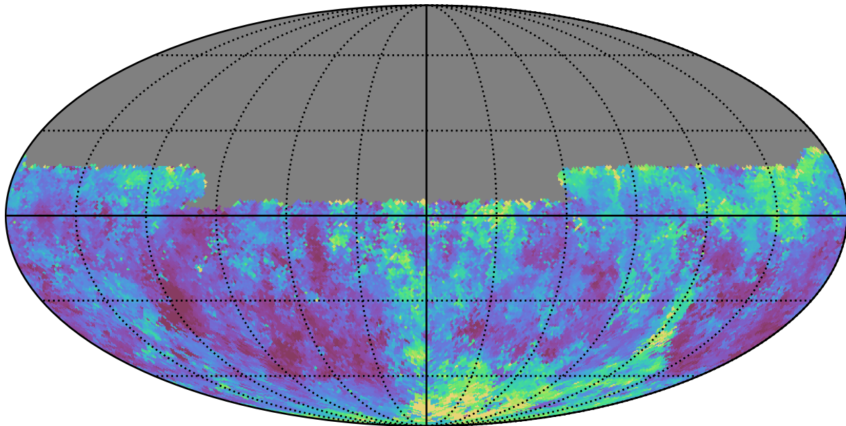
too_10_1v3.4_10yrs Yr 1 y band: Median seeingEff
