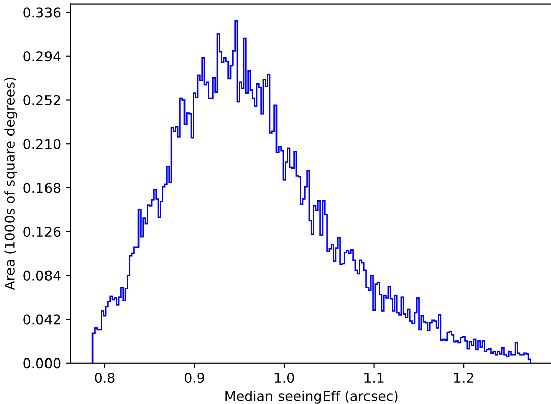
too_10_1v3.4_10yrs Yr 1 y band: Median seeingEff
