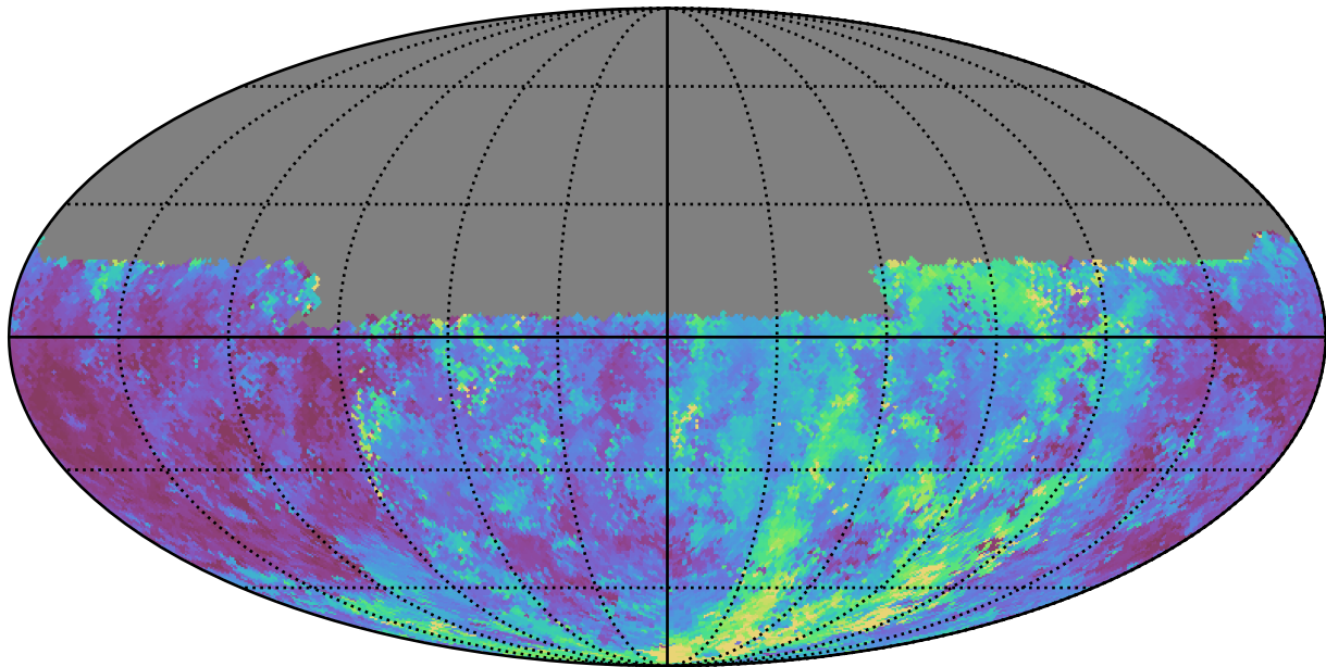
too_10_1v3.4_10yrs Yr 1 u band: Median seeingEff
