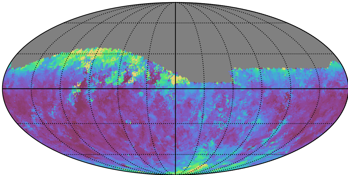
too_10_1v3.4_10yrs Yr 1 r band: Median seeingEff
