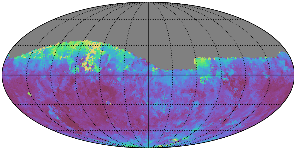
too_10_1v3.4_10yrs Yr 1 i band: Median seeingEff
