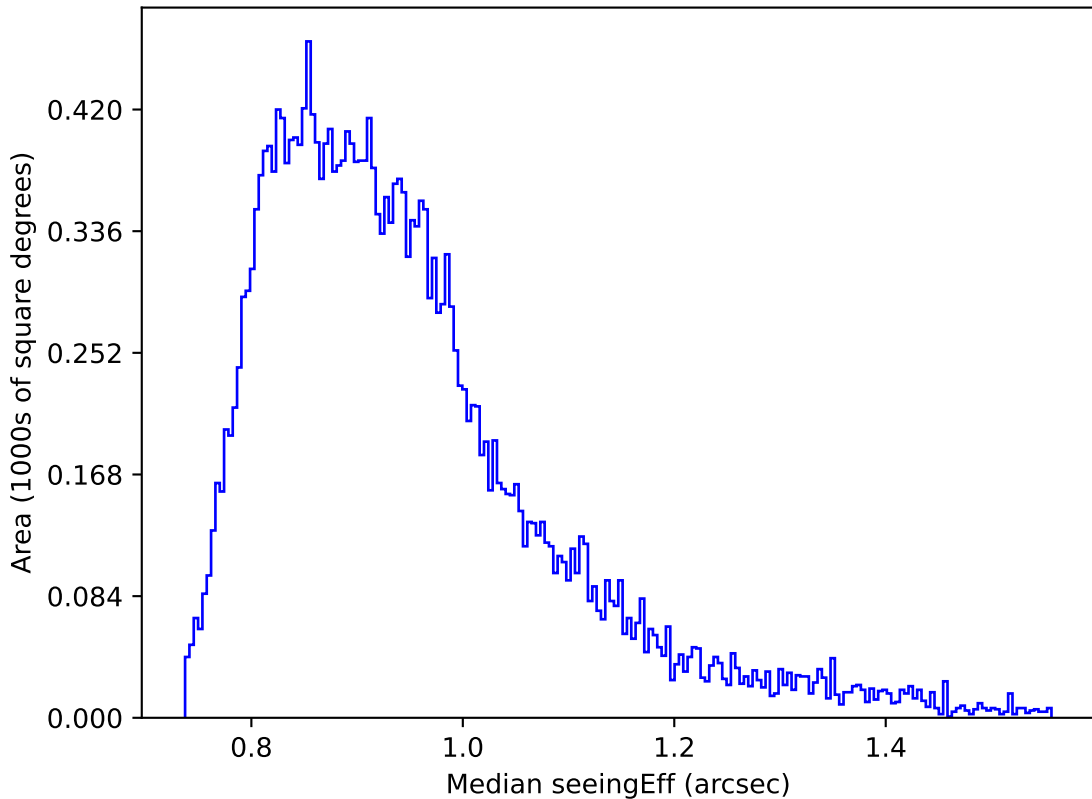
too_10_1v3.4_10yrs Yr 1 i band: Median seeingEff
