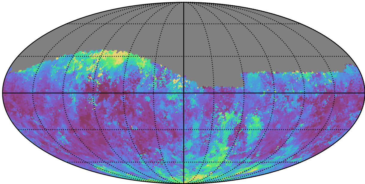
too_10_1v3.4_10yrs Yr 1 g band: Median seeingEff
