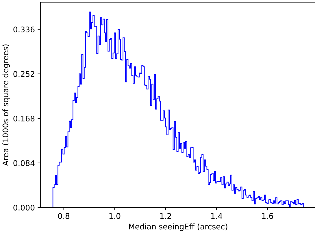
too_10_1v3.4_10yrs Yr 1 g band: Median seeingEff
