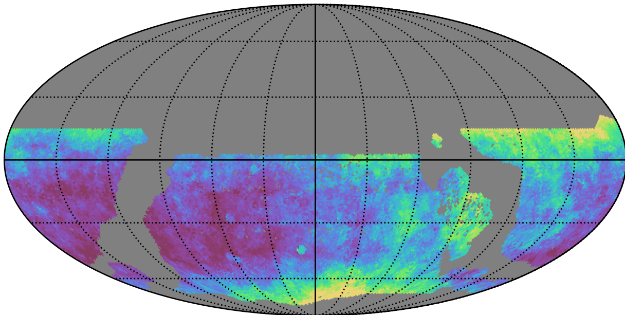
too_10_1v3.4_10yrs WFD y band: Median seeingEff
