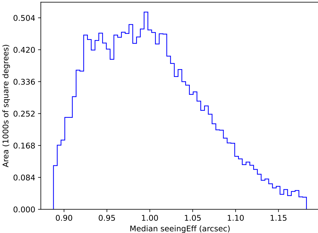
too_10_1v3.4_10yrs WFD y band: Median seeingEff
