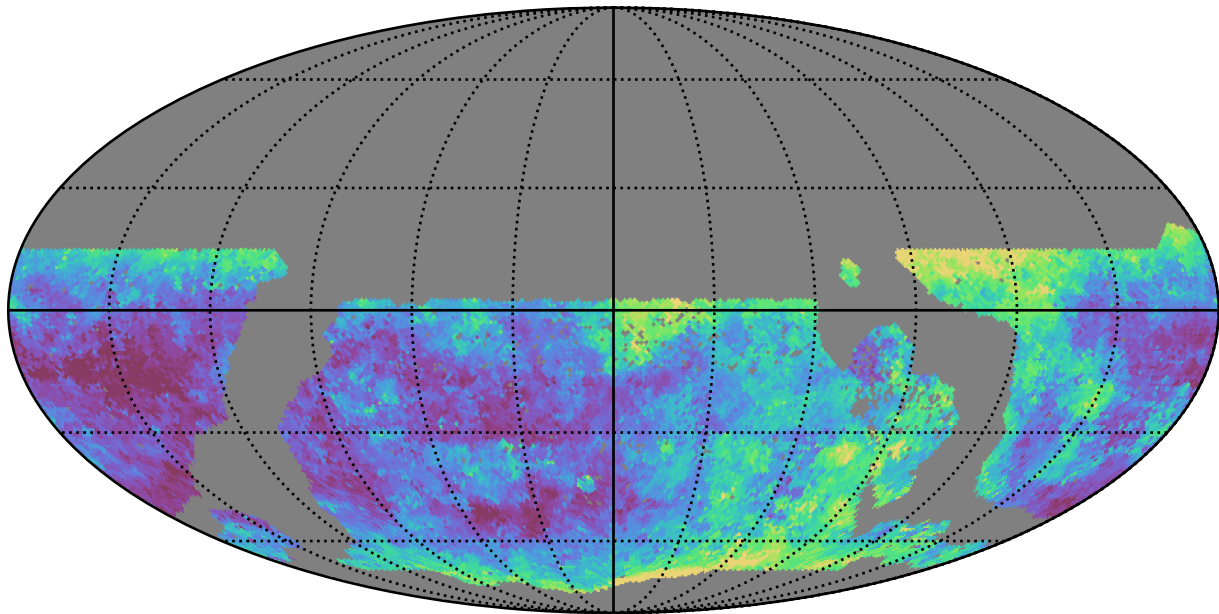
too_10_1v3.4_10yrs WFD u band: Median seeingEff
