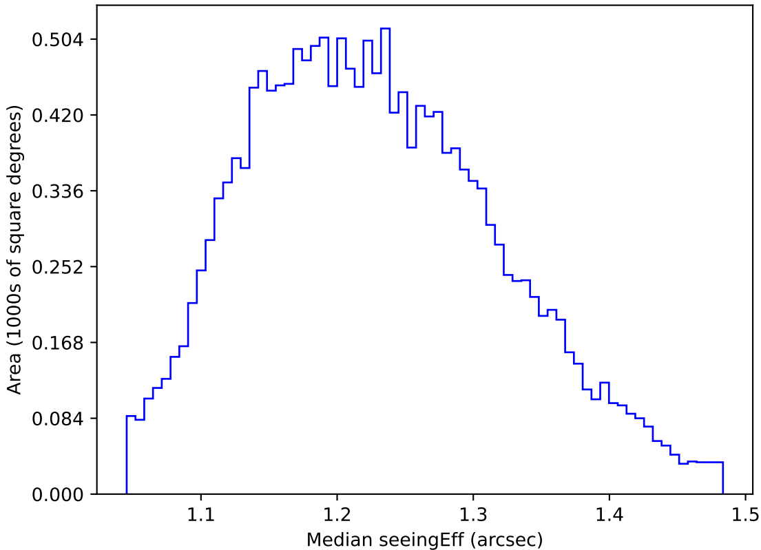
too_10_1v3.4_10yrs WFD u band: Median seeingEff
