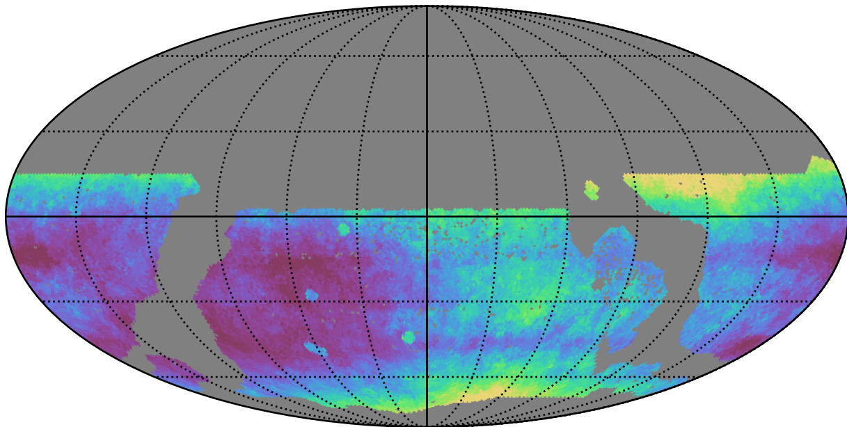
too_10_1v3.4_10yrs WFD r band: Median seeingEff
