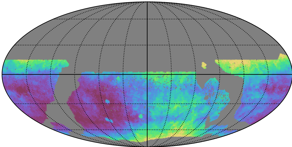
too_10_1v3.4_10yrs WFD i band: Median seeingEff
