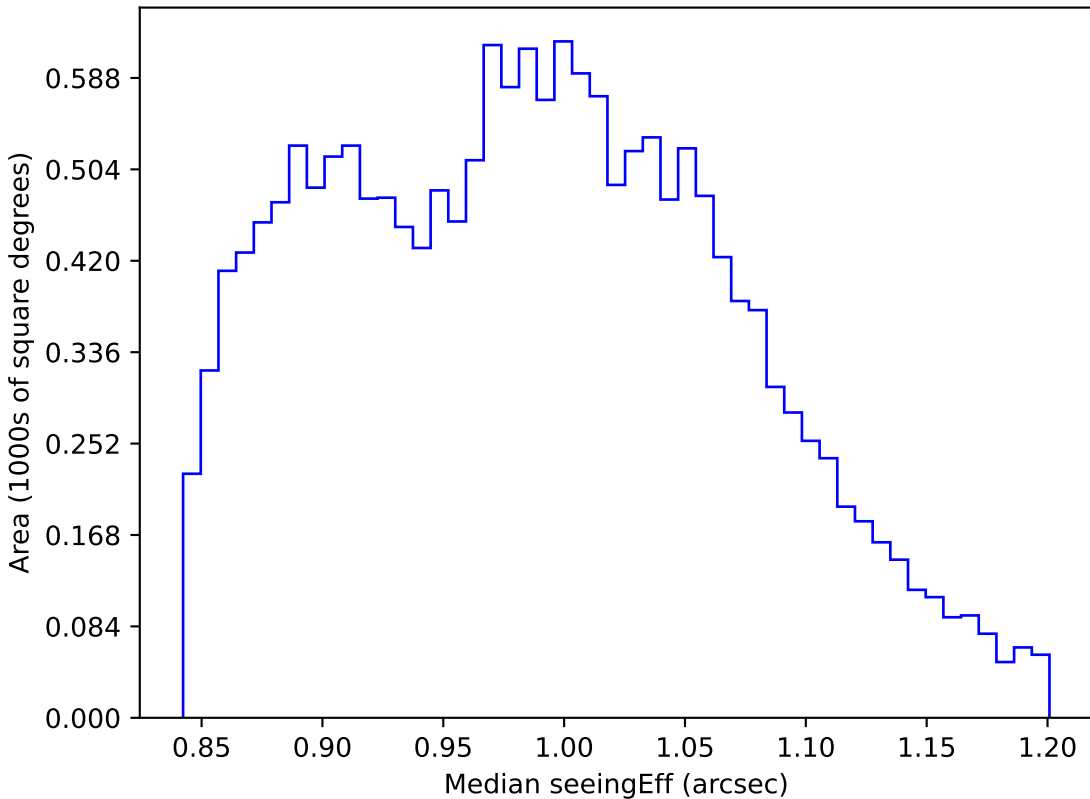
too_10_1v3.4_10yrs WFD i band: Median seeingEff
